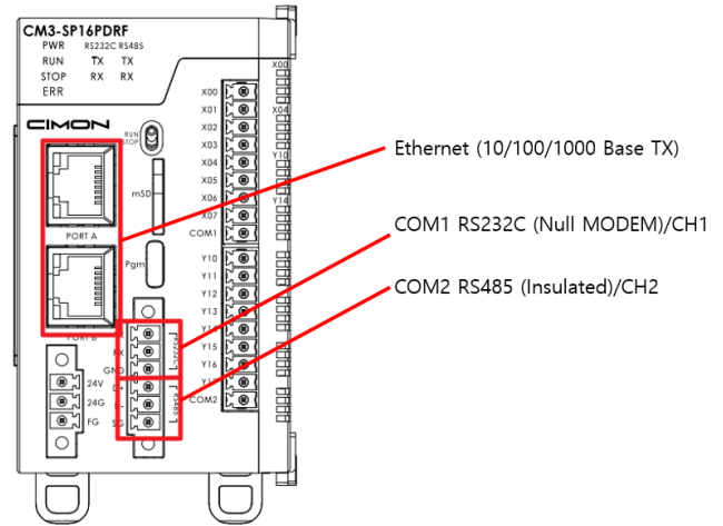
CM3-SP16PDRF Input - Output
